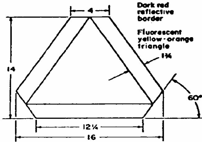
FIGURE J-7.—SLOW-MOVING VEHICLE EMBLEM
